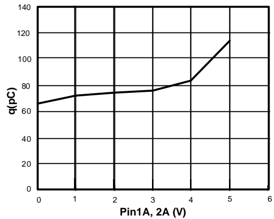
Charge Injection vs. Pin1A, 2A Voltage
