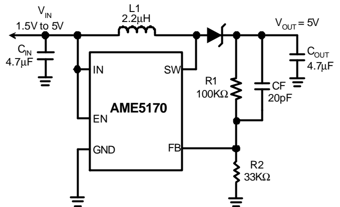
Figure.1 Typical 5V Application
