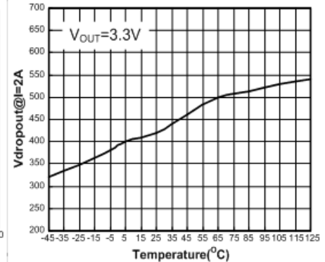
Vdropout@I=2A vs. Temperature
