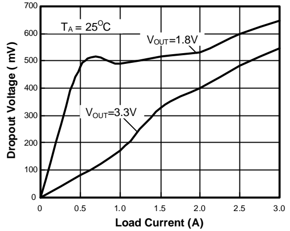
Dropout Voltage vs. Load Current (For TO-263 Package)
