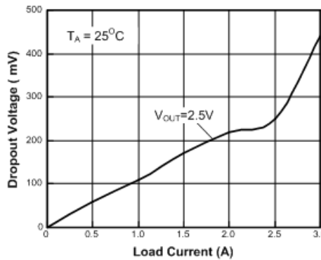
Dropout Voltage v.s Load Current (TO-252)
