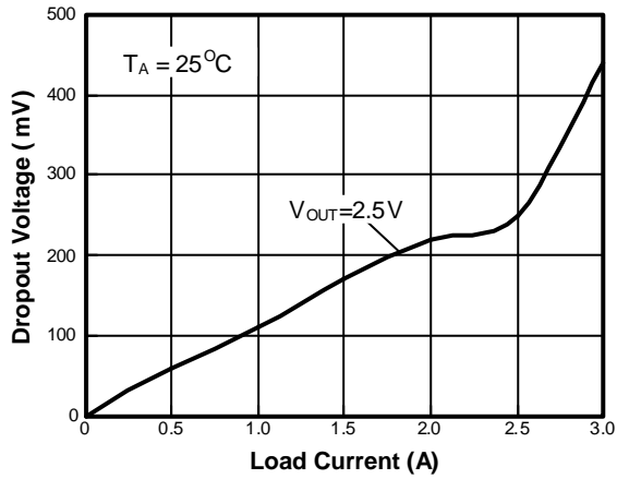
Dropout Voltage vs. Load Current (For TO-252 Package)
