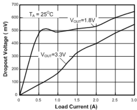
Dropout Voltage v.s Load Current (TO-263)
