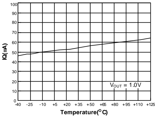
Quiescent Current
