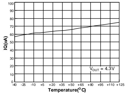
Quiescent Current
