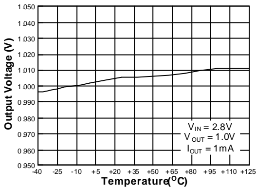
Output Voltage
