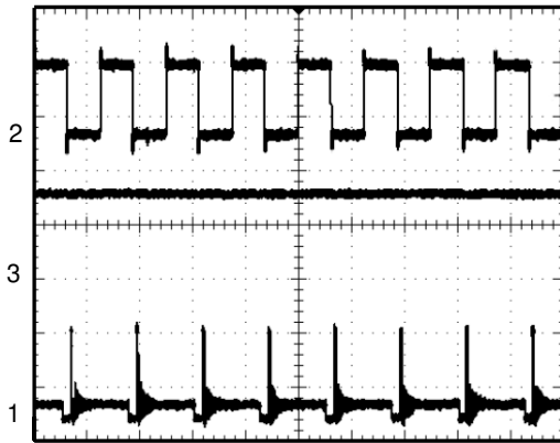
Dimming Control for Driving 6LEDs
