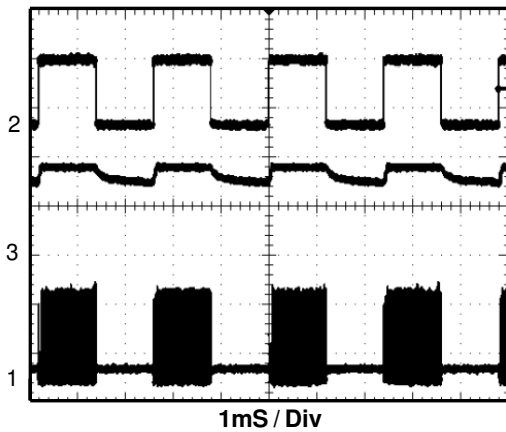
Dimming Control for Driving 6LEDs
