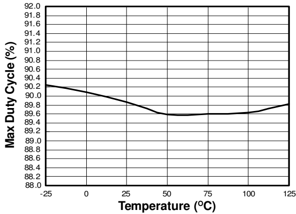
Max Duty Cycle vs. Temperature
