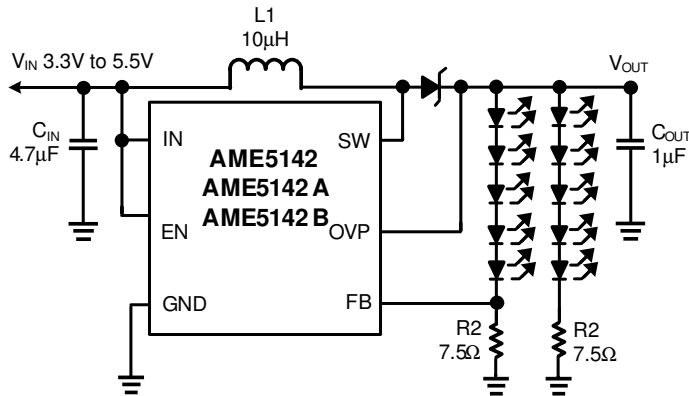
Figure 14: Circuit For Driving 2 Strings of 5 White LEDs
