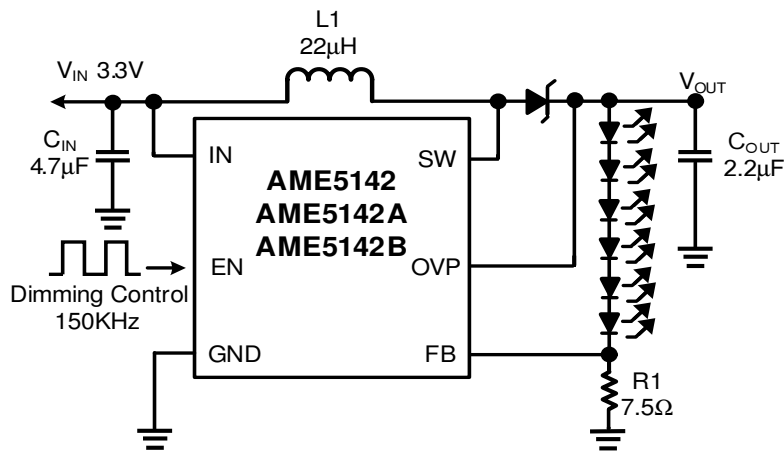
Figure 5. PWM Dimming Control Using the EN Pin
