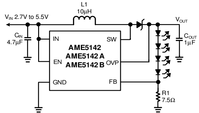
Figure 2: Circuit For Driving 4 White LEDs
