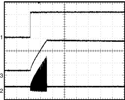
Start up into Openload AME5142B
