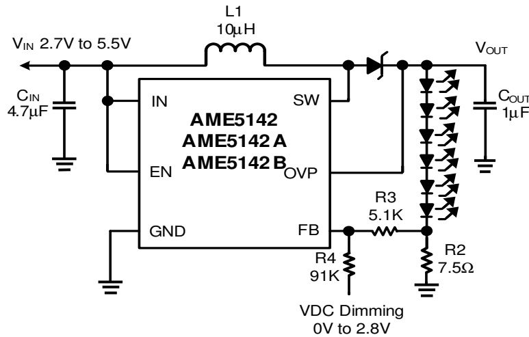
Figure 6. Dimming Control Using a DC Voltage
