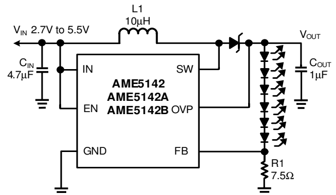
Figure 3: Circuit For Driving 6 White LEDs
