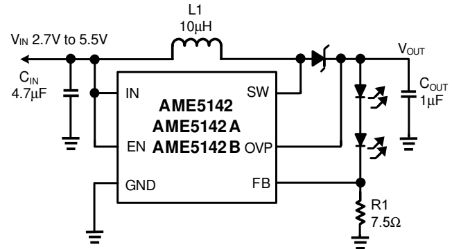
Figure 1: Circuit For Driving 2 White LEDs
