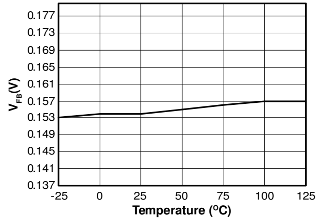
V_{FB} vs. Temperature
