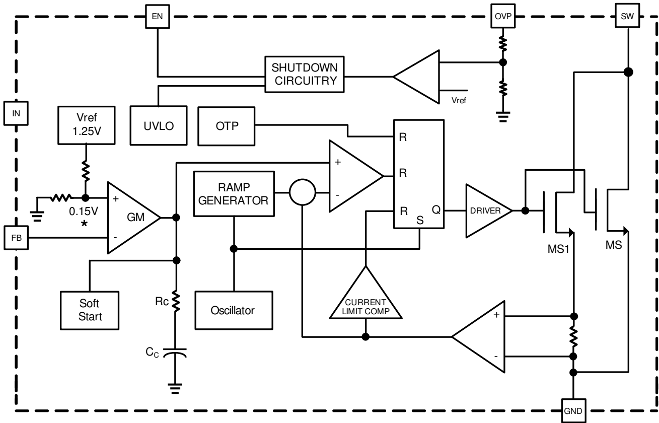
Figure 4 : AME5142/5142A/5142B Block Diagram
