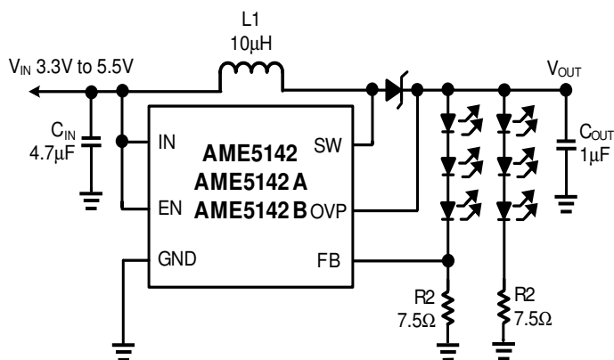
Figure 10: Circuit For Driving 2 Strings of 3 White LEDs
