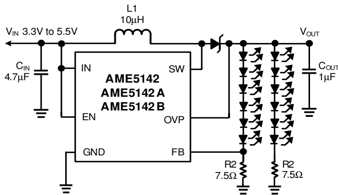
Figure 15: Circuit For Driving 2 Strings of 6 White LEDs
