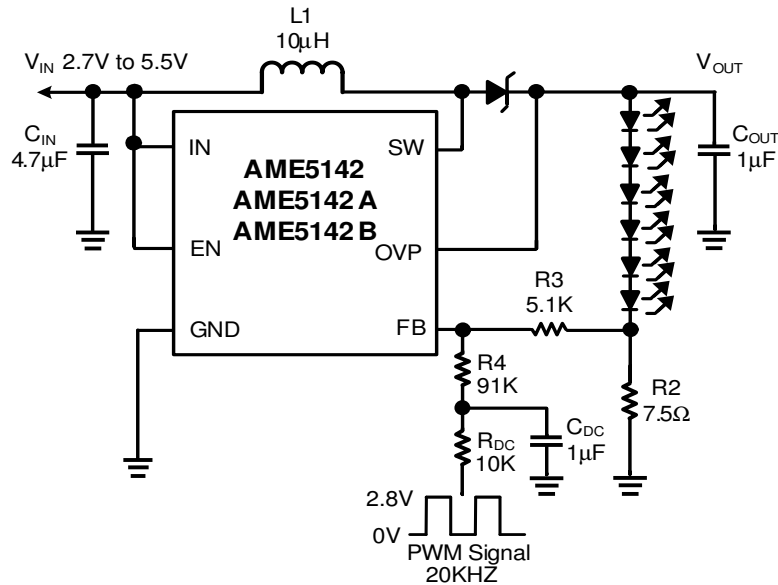
Figure 7. Dimming Control Using a Filtered PWM Signal
