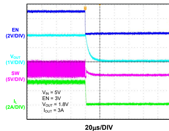
Power Off_EN
