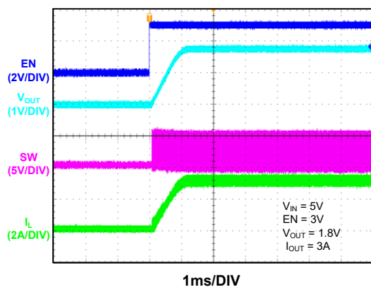
Power On_EN
