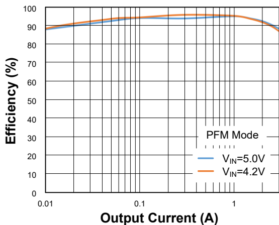
Efficiency vs. Output Current_3.3V
