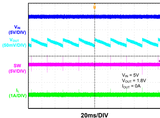
Steady State
